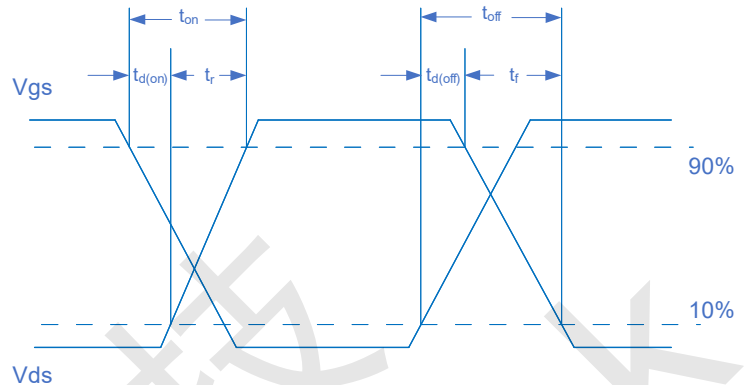
Figure 2 Switching Waveform
