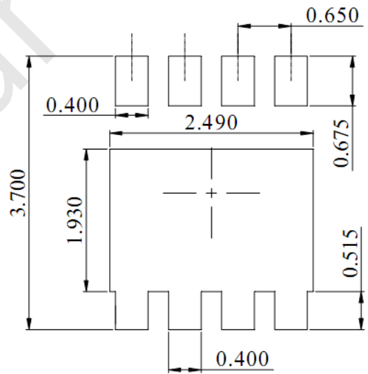
DIMENSIONS:MILLIMETERS
