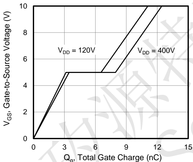
Figure 9. Gate Charge
