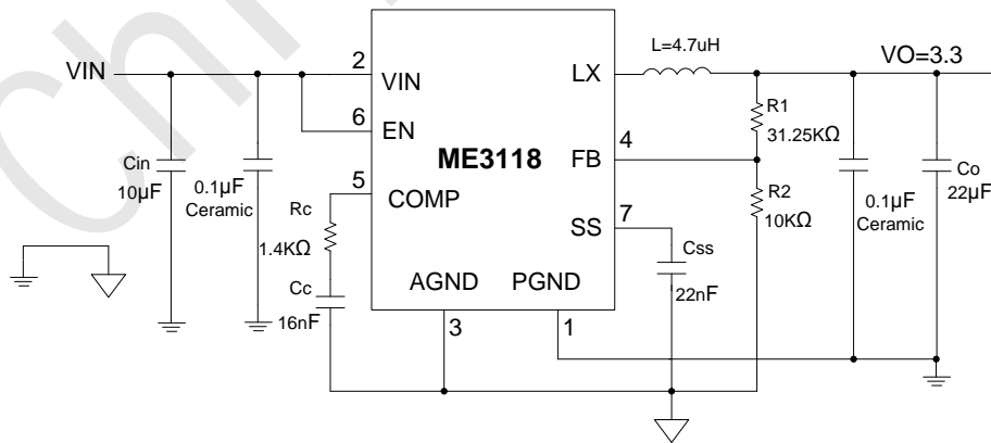
Fig.1 3.3V 3A同步整流降压, F_s = 500 \text{ KHz}
