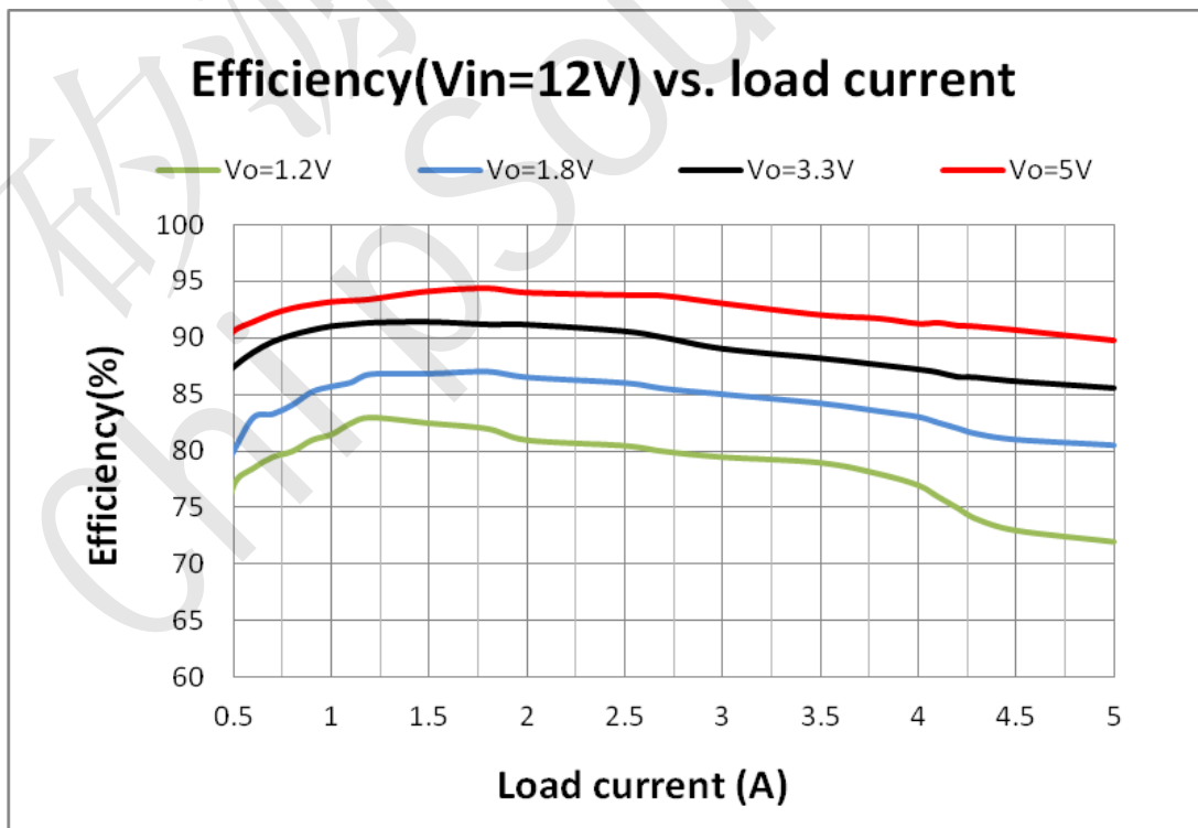
Fig.3 Efficiency2 (Vin=12V)
