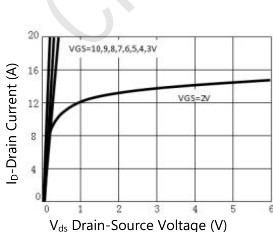
Figure 5. Output Characteristics
