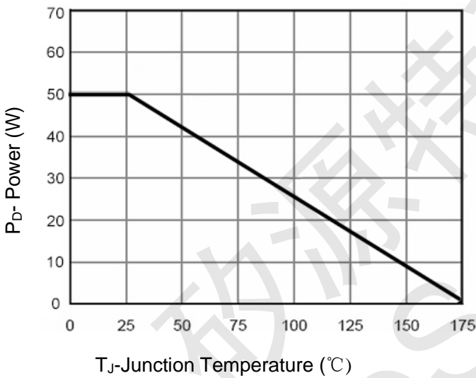
Figure 3 Power De-rating
