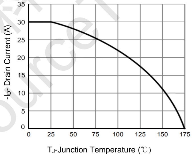
Figure 4 Drain Current
