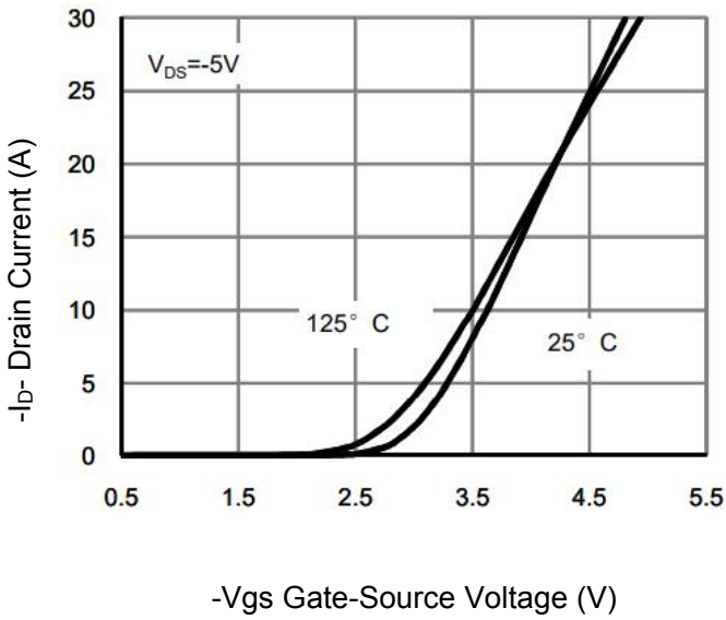
Figure 7 Transfer Characteristics
