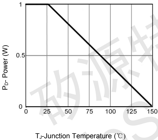
Figure 3 Power Dissipation
