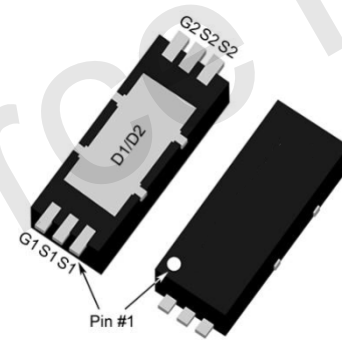
PDFN2x5-6L
