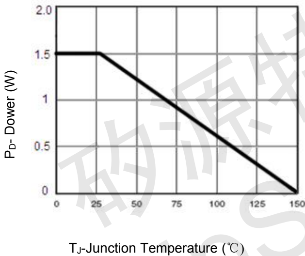
Figure 3 Power Dissipation
