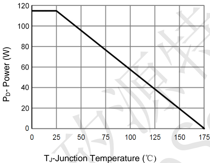
Figure 3 Power De-rating
