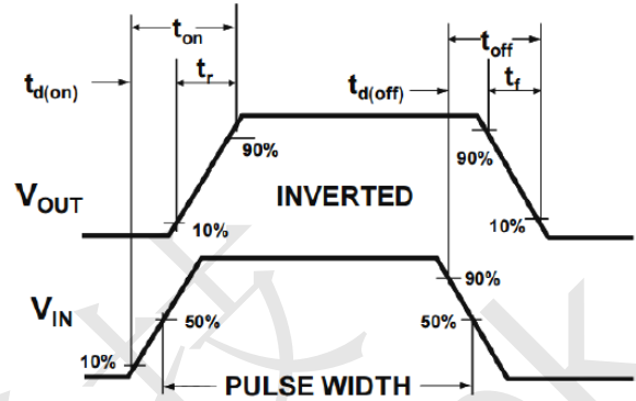
Figure 2 Switching Waveform
