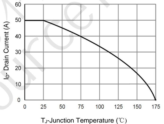
Figure 4 Drain Current
