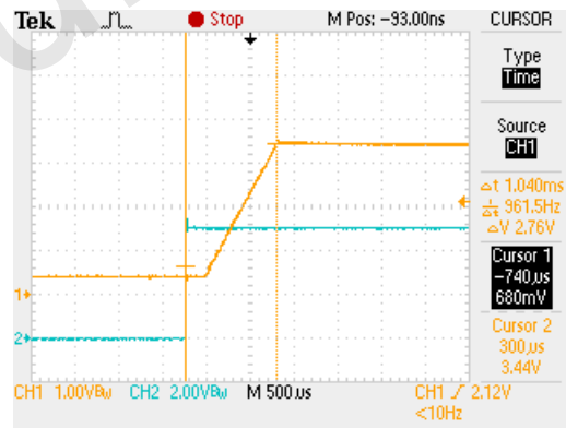
STRAT UP (V IN =5V, V OUT =3.3V)
