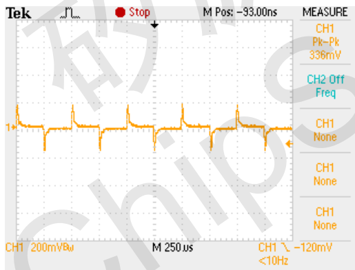
LOAD TRANSIENT RESPONSE (V IN =5V, V OUT =3.3V, I OUT =500-1500mA, 1A/μS)
