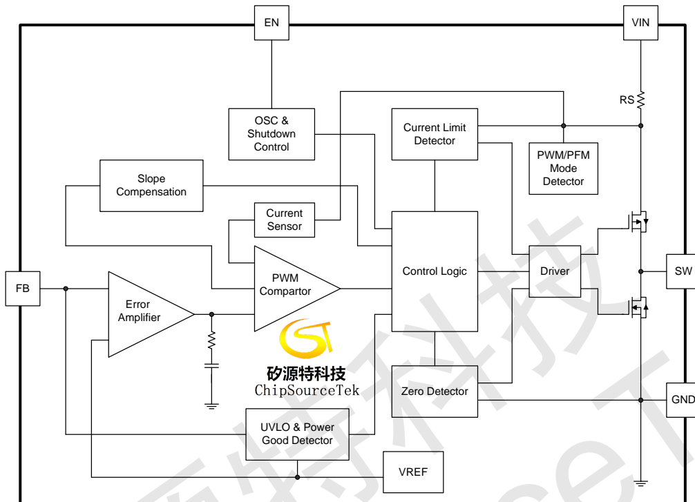
Figure 1. RY3420 Block Diagram
