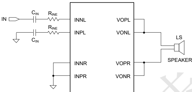
Figure 11. PBTB Configuration for Mono Applications
