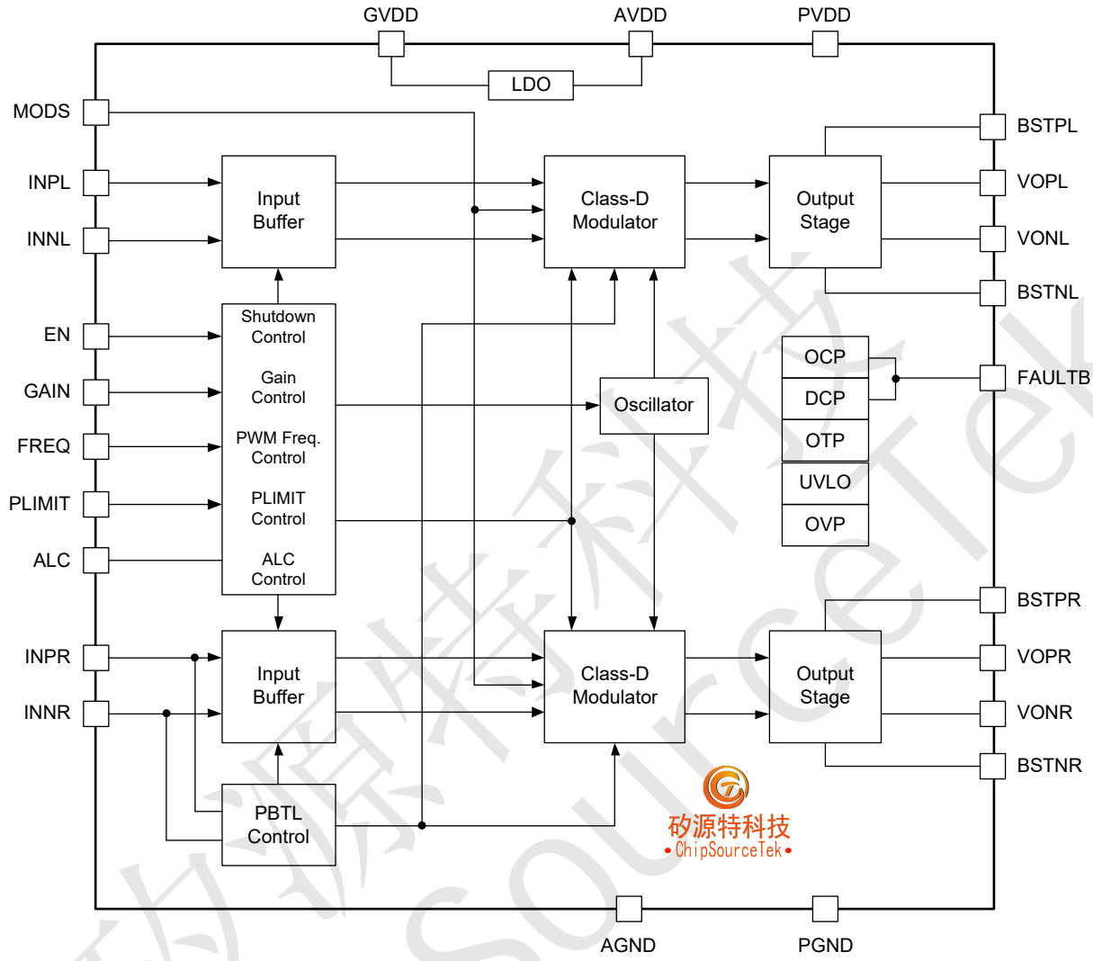
Figure 3. Block Diagram
