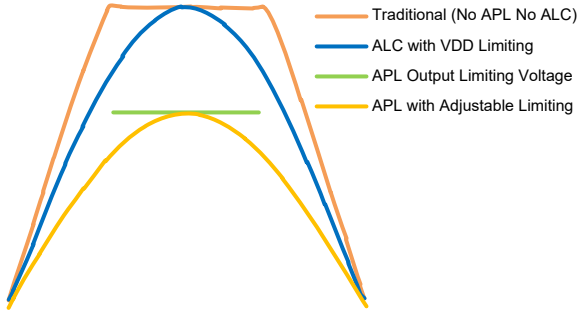
Figure 4. Large Audio Outputs in Different Operating Modes
