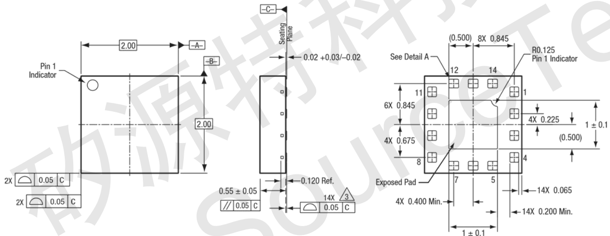
Figure 4. FM3418 14-Pin QFN Package Dimensions
