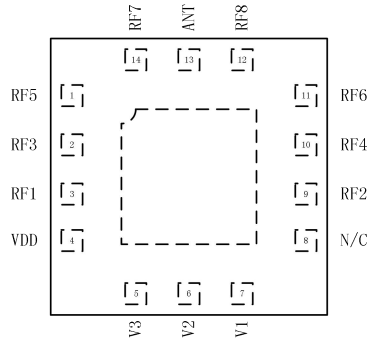
Figure 2. FM3418 Pinout - 14-Pin QFN (Top View)
