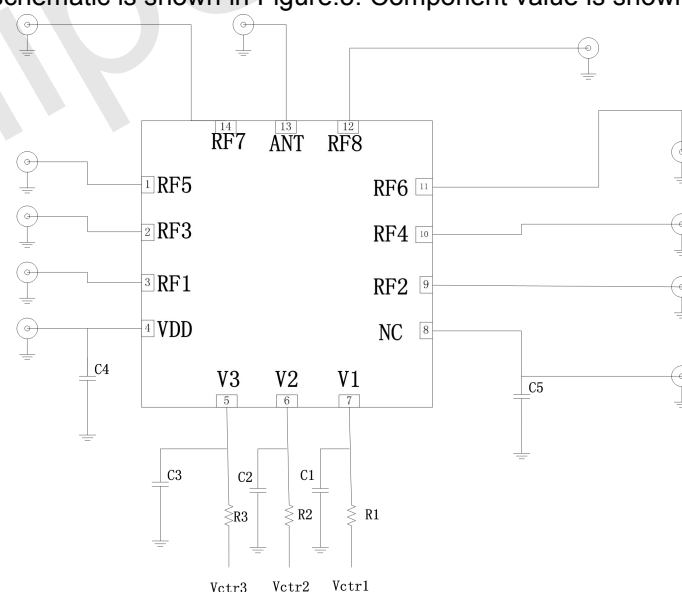
Figure 3. FM3418 Application Schematic
