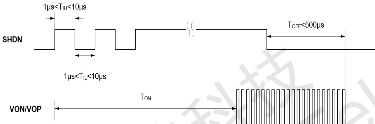
Figure 1. Single Wire Pulse Control Timing Sequence
