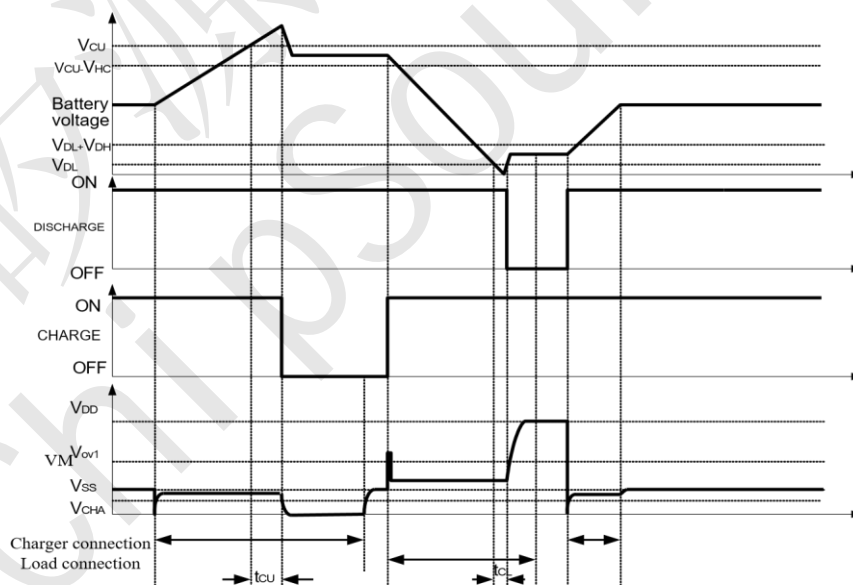
Figure5-1 Overcharge and Overdischarge Voltage Detection
