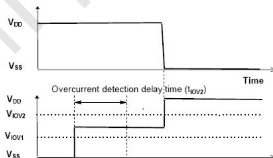
Figure 4. Overcurrent delay time
