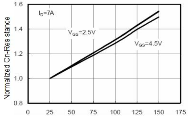
Figure 4 Drain-Source On-Resistance
