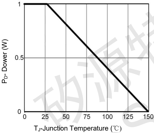
Figure 3 Power De-rating
