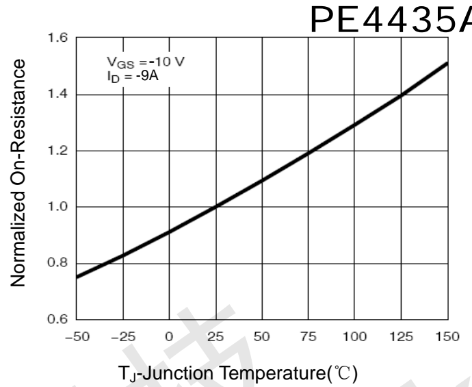
Figure 8 Drain-Source On-Resistance
