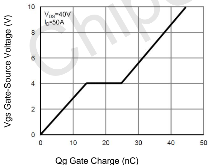
Figure 11 Gate Charge
