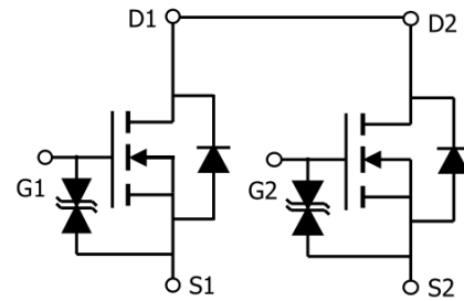
Schematic diagram
