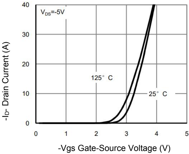
Figure 7 Transfer Characteristics
