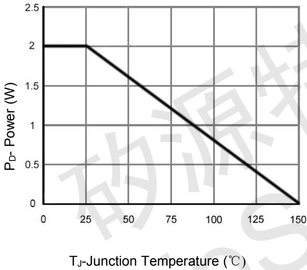
Figure 3 Power De-rating
