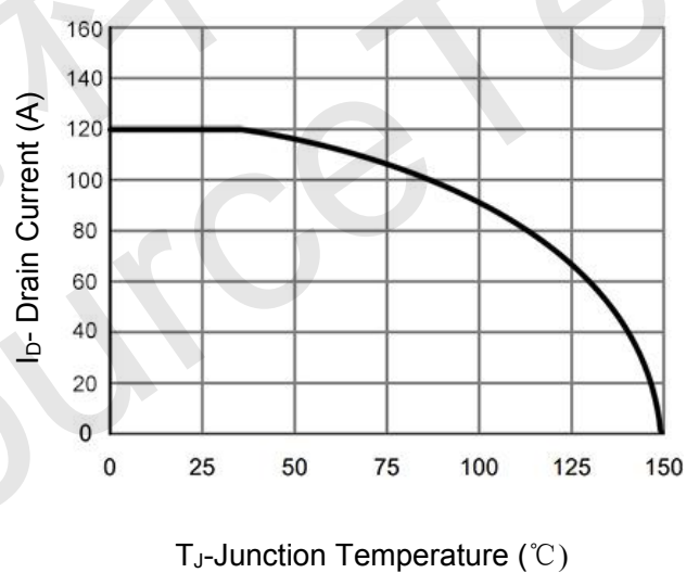
Figure 4 Drain Current
