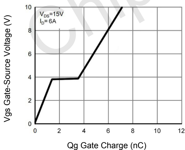
Figure 11 Gate Charge
