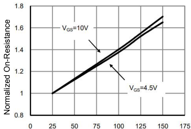
T J -Junction Temperature(°C) Figure 8 Rdson vs Junction Temperature
