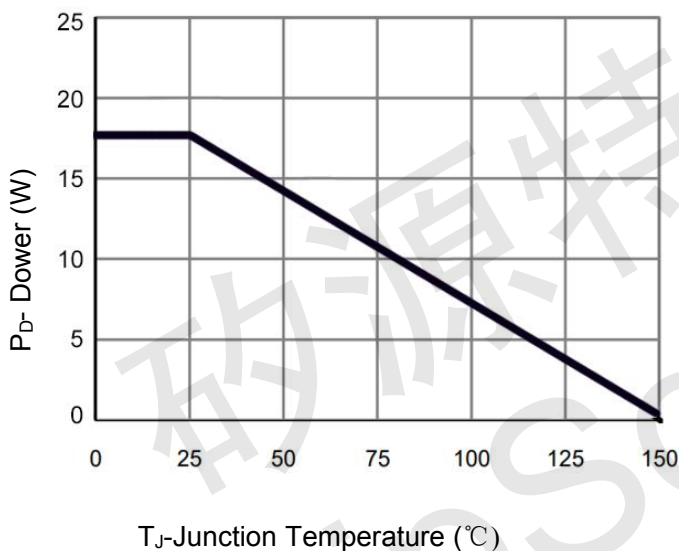
Figure 3 Power De-rating
