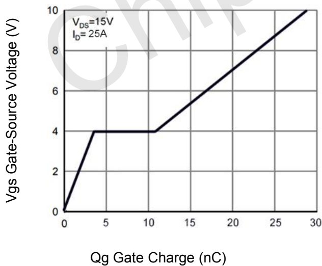
Figure 11 Gate Charge
