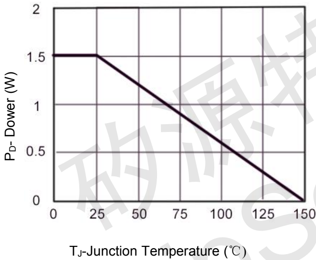
Figure 3 Power Dissipation
