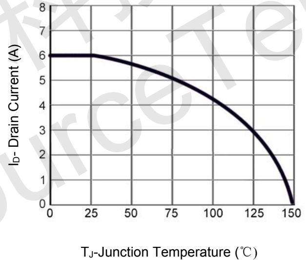
Figure 4 Drain Current
