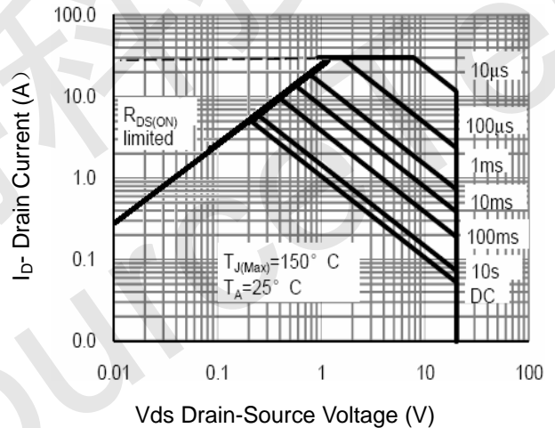
Figure 4 Safe Operation Area
